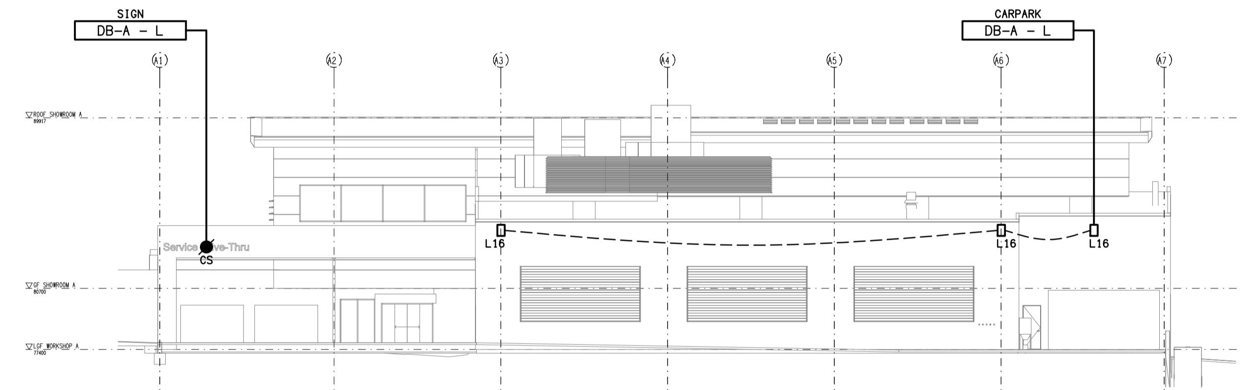
SOUTHERN ELEVATION
