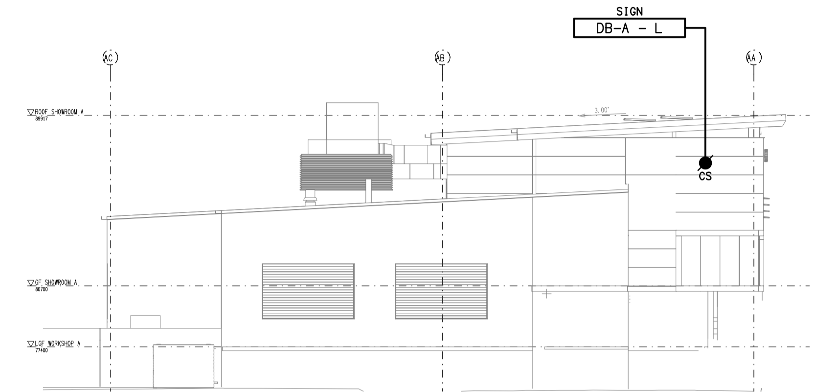
EASTERN ELEVATION
